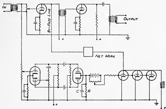
FIG. 6. Selective by-pass circuit.
